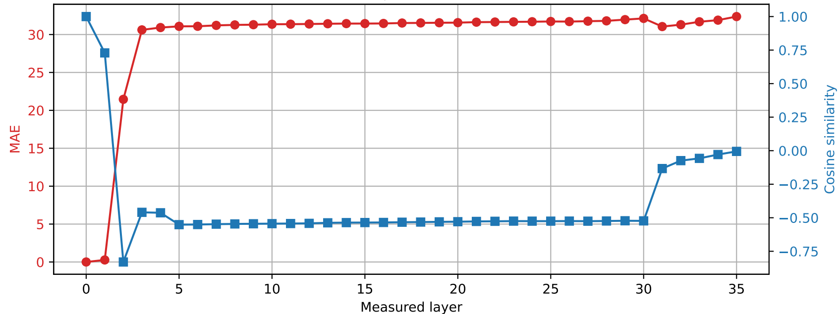
Qwen2.5-3B | Prompt 0 Spared layer 33 | Hybrid vs unquantized
