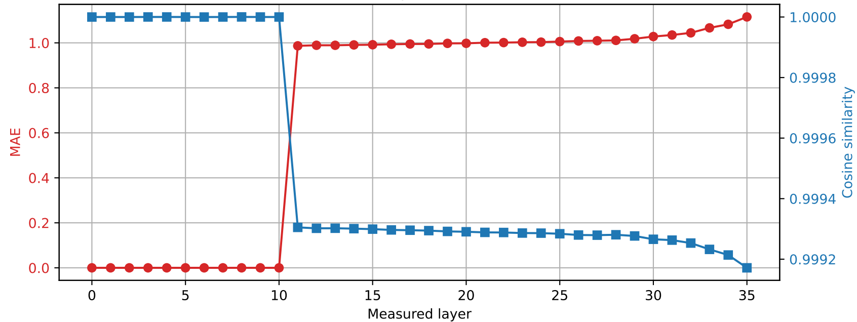
Qwen2.5-3B | Prompt 1 Spared layer 10 | Hybrid vs quantized
