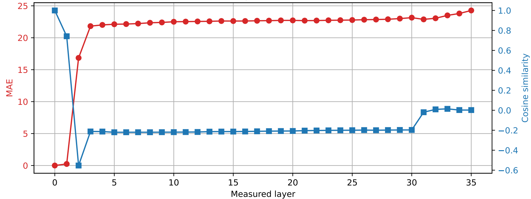
Qwen2.5-3B | Prompt 1 Spared layer 20 | Hybrid vs unquantized
