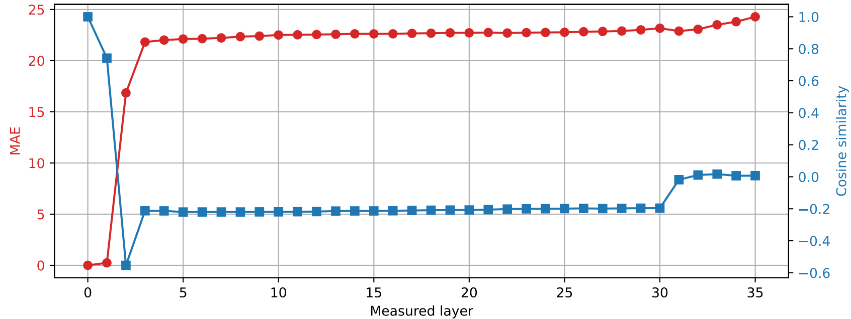
Qwen2.5-3B | Prompt 1 Spared layer 21 | Hybrid vs unquantized
