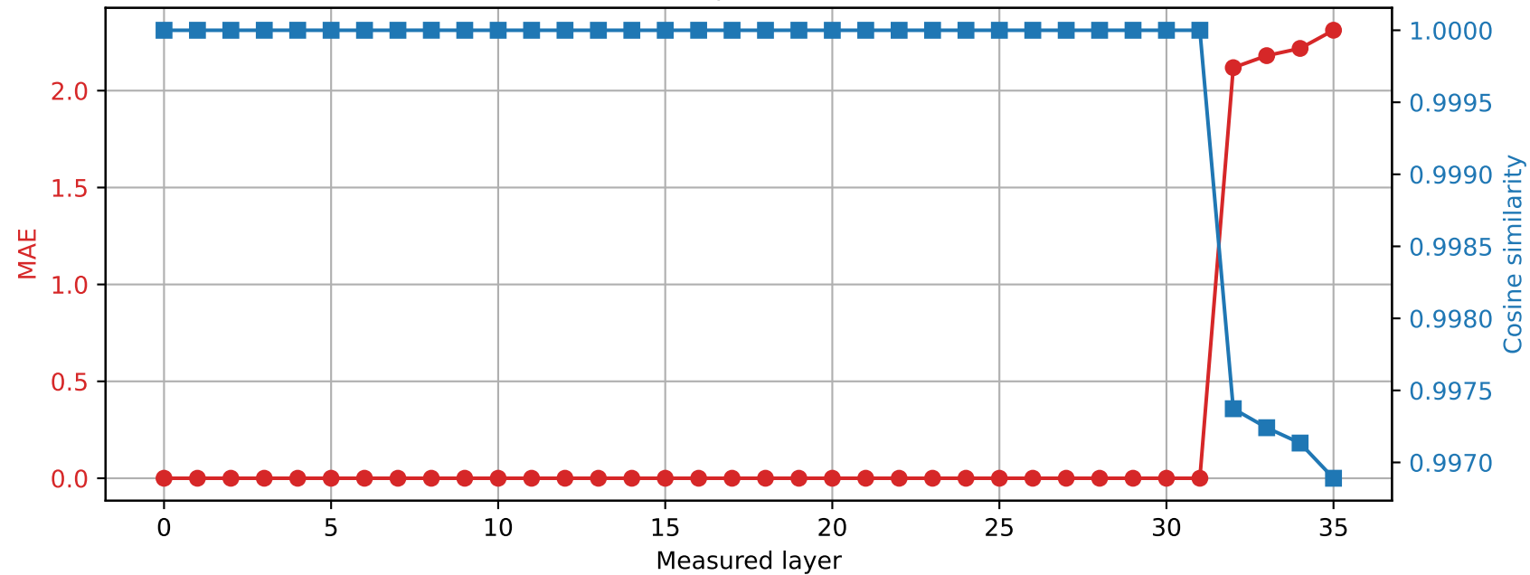
Qwen2.5-3B | Prompt 1 Spared layer 31 | Hybrid vs quantized
