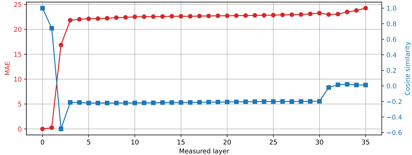
Qwen2.5-3B | Prompt 1 Spared layer 31 | Hybrid vs unquantized
