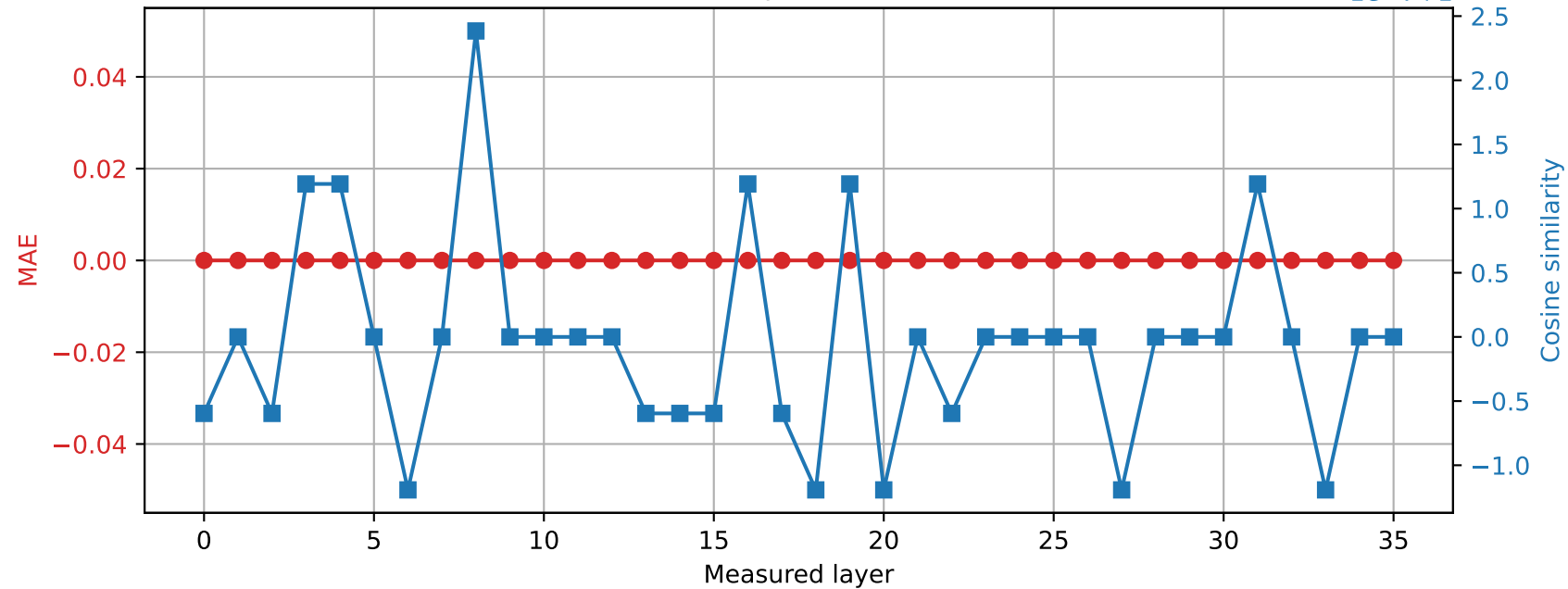
Qwen2.5-3B | Prompt 1 Spared layer 35 | Hybrid vs quantized
