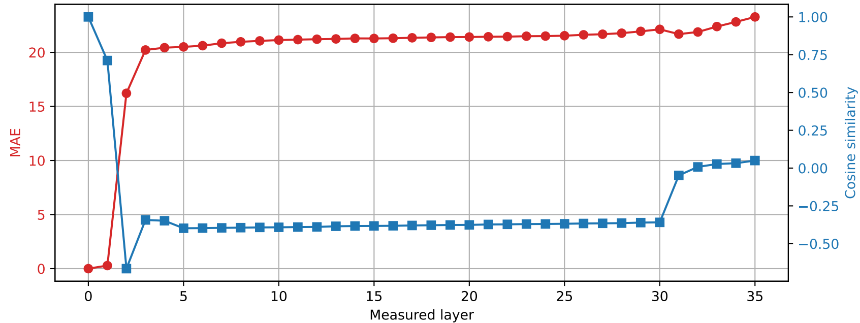
Qwen2.5-3B | Prompt 2 Unquantized vs quantized int4
