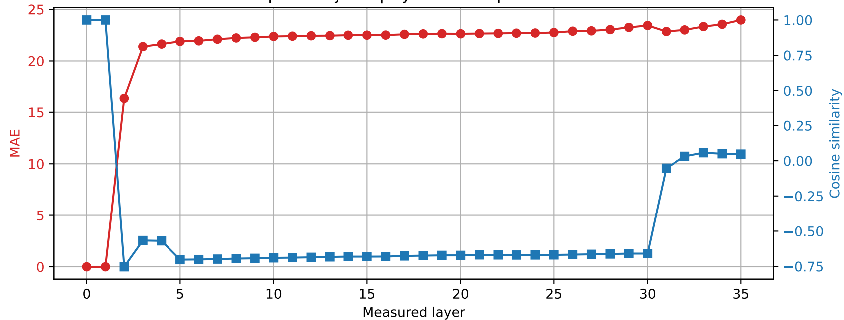
Qwen2.5-3B | Prompt 2 Spared layer 0 | Hybrid vs unquantized
