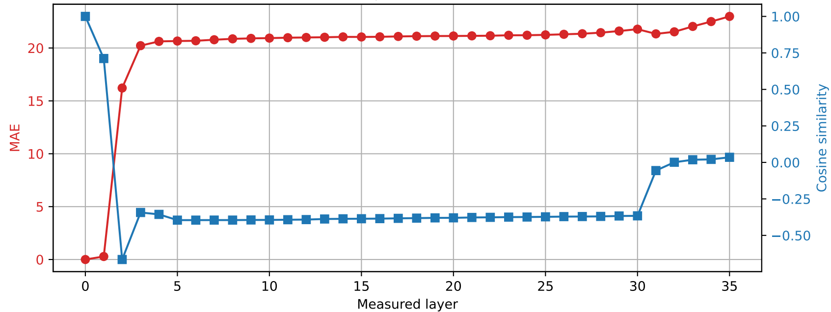
Qwen2.5-3B | Prompt 2 Spared layer 3 | Hybrid vs unquantized
