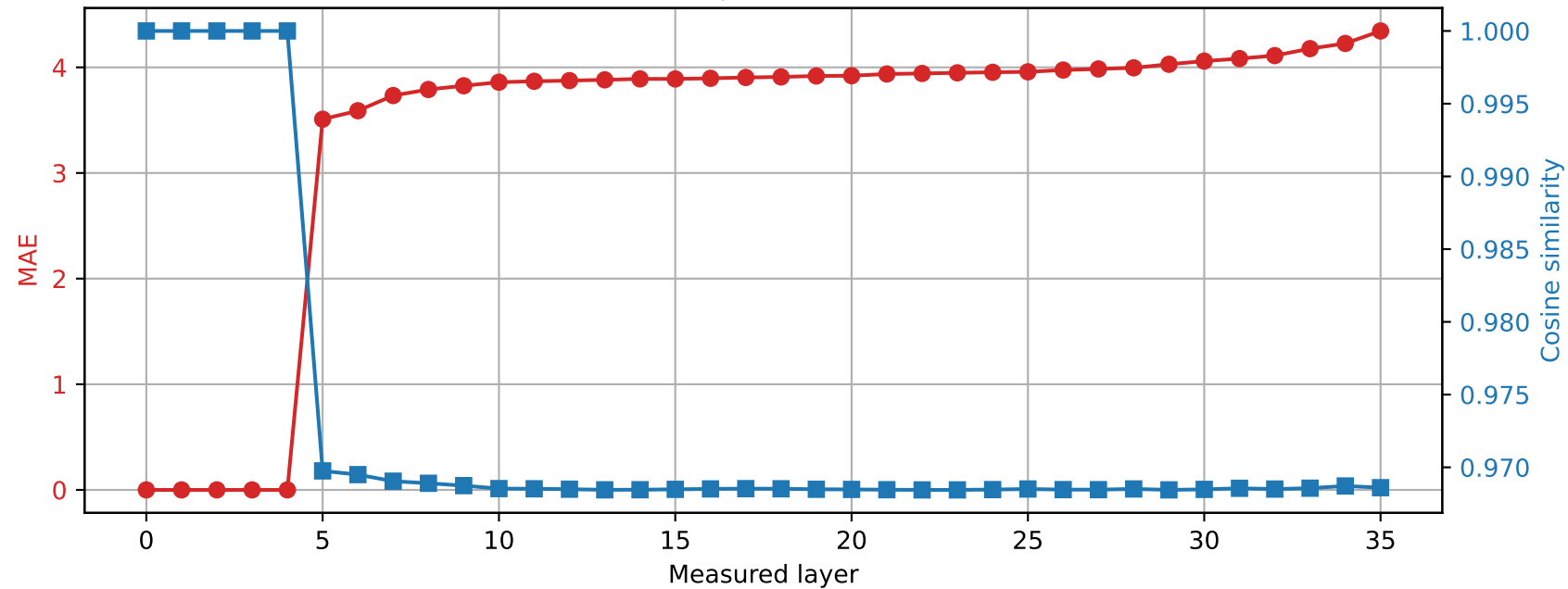
Qwen2.5-3B | Prompt 2 Spared layer 4 | Hybrid vs quantized
