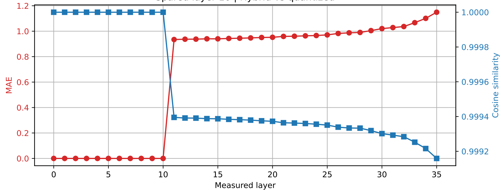
Qwen2.5-3B | Prompt 2 Spared layer 10 | Hybrid vs quantized
