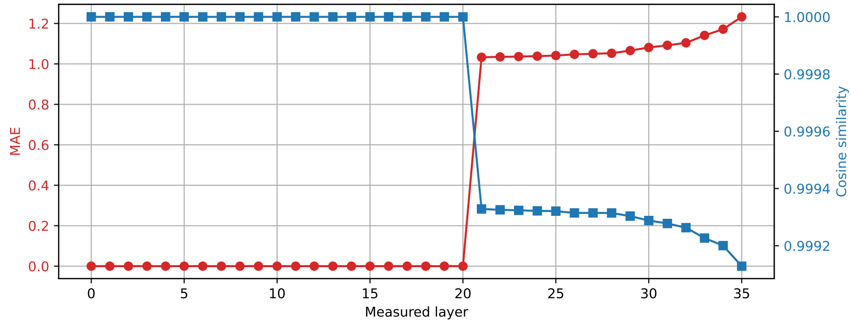
Qwen2.5-3B | Prompt 2 Spared layer 20 | Hybrid vs quantized
