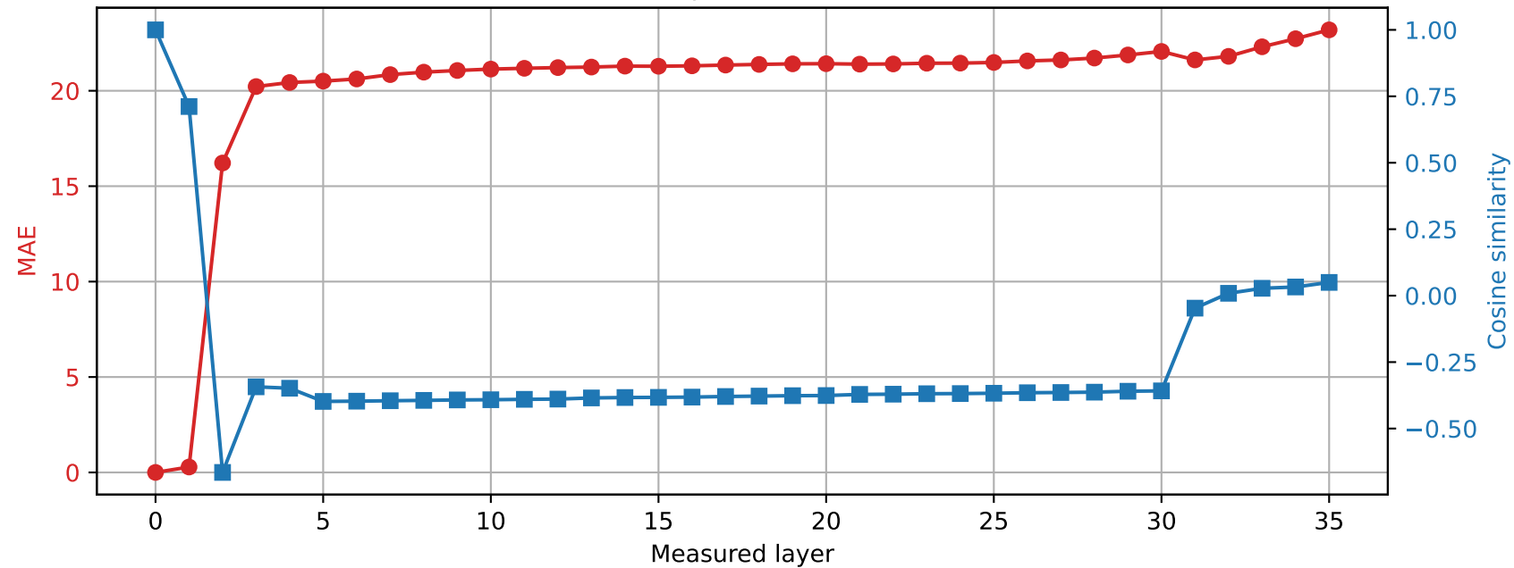
Qwen2.5-3B | Prompt 2 Spared layer 20 | Hybrid vs unquantized
