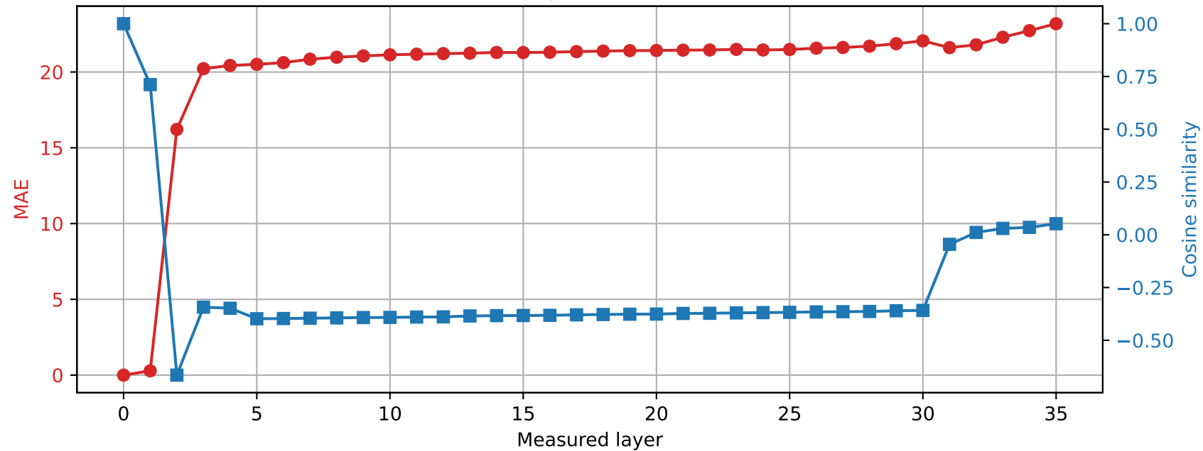
Qwen2.5-3B | Prompt 2 Spared layer 23 | Hybrid vs unquantized
