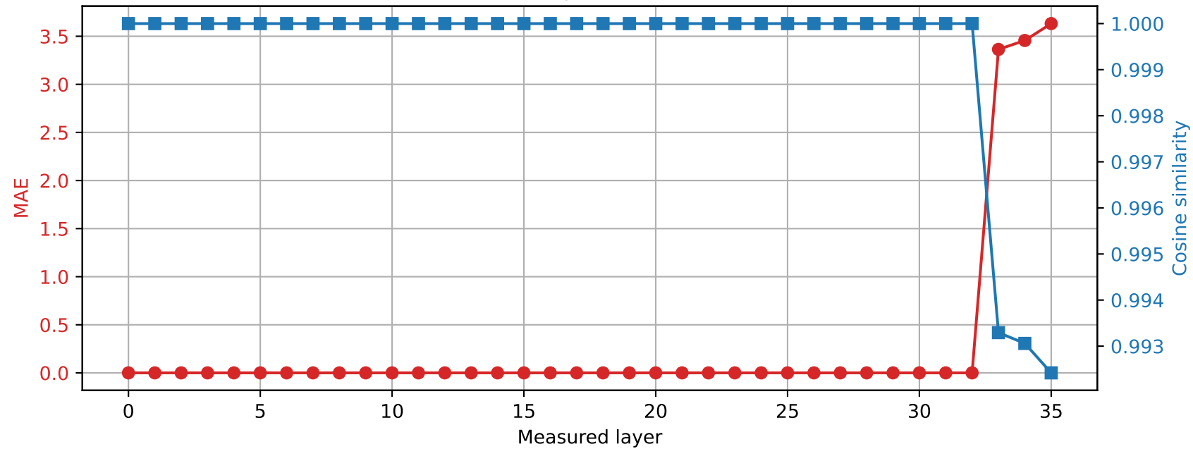
Qwen2.5-3B | Prompt 2 Spared layer 32 | Hybrid vs quantized
