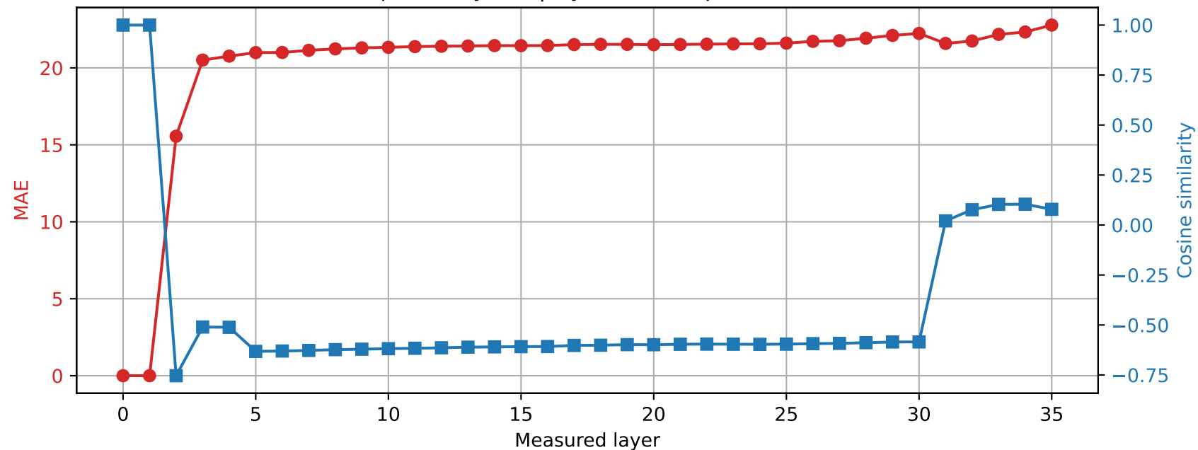
Qwen2.5-3B | Prompt 3 Spared layer 0 | Hybrid vs unquantized
