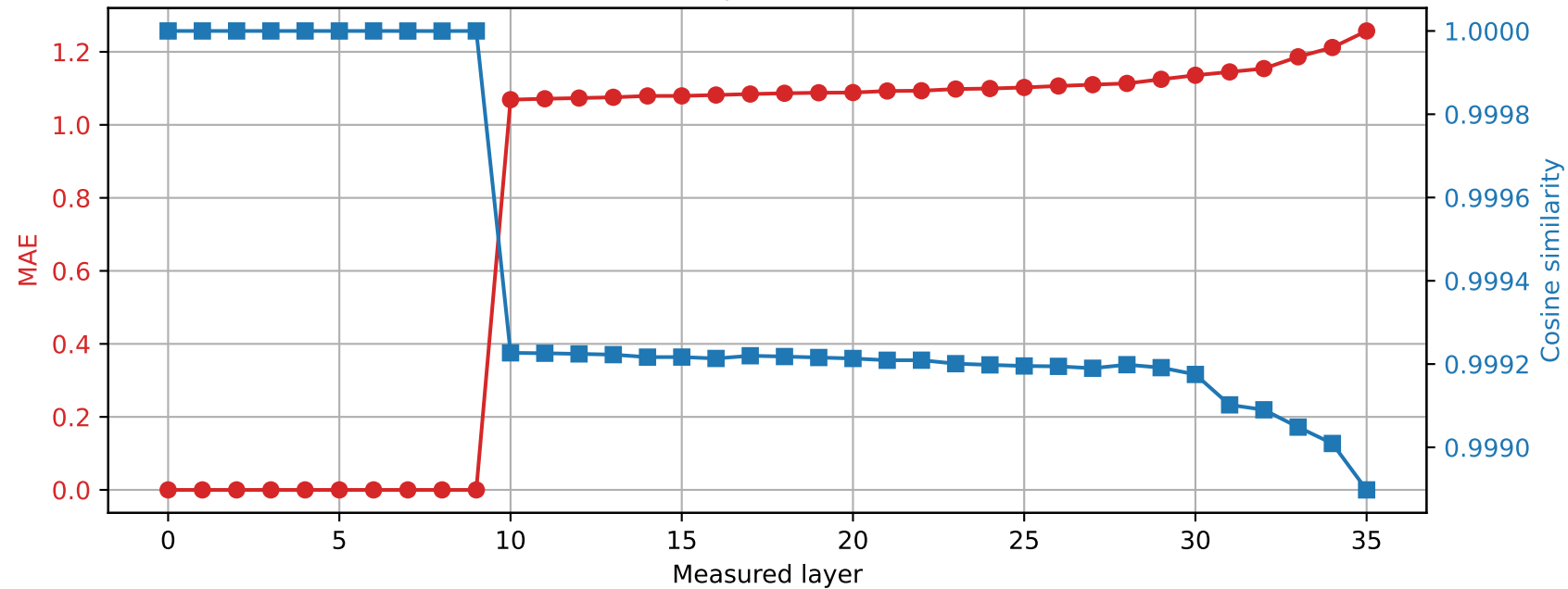
Qwen2.5-3B | Prompt 3 Spared layer 9 | Hybrid vs quantized
