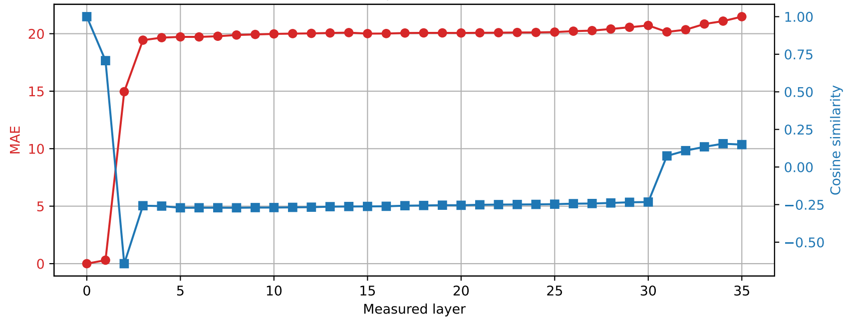
Qwen2.5-3B | Prompt 3 Spared layer 14 | Hybrid vs unquantized
