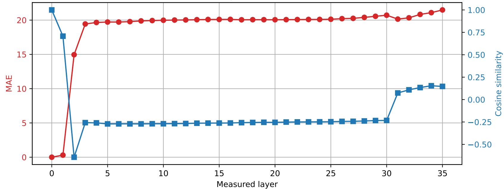
Qwen2.5-3B | Prompt 3 Spared layer 16 | Hybrid vs unquantized
