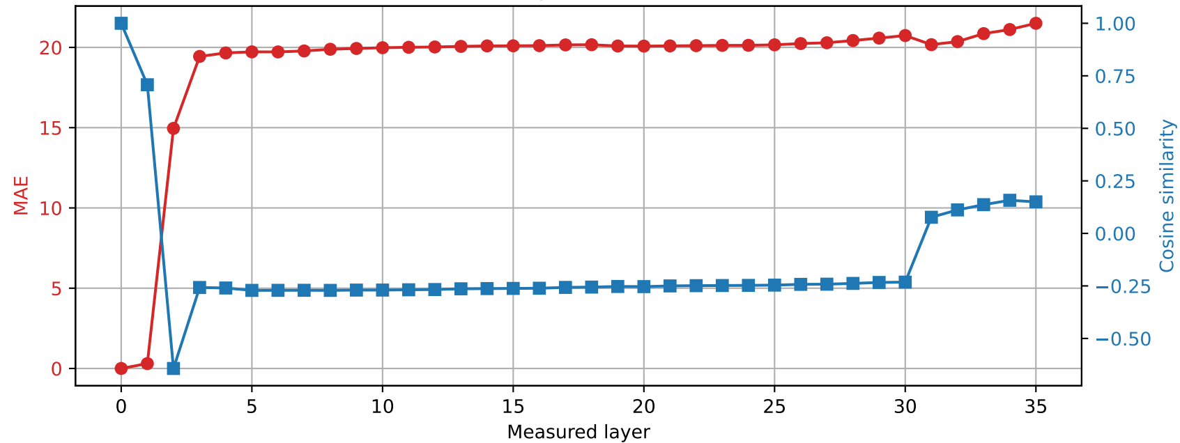
Qwen2.5-3B | Prompt 3 Spared layer 18 | Hybrid vs unquantized
