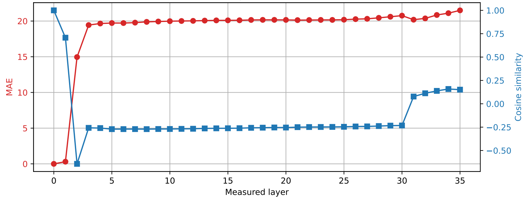
Qwen2.5-3B | Prompt 3 Spared layer 20 | Hybrid vs unquantized
