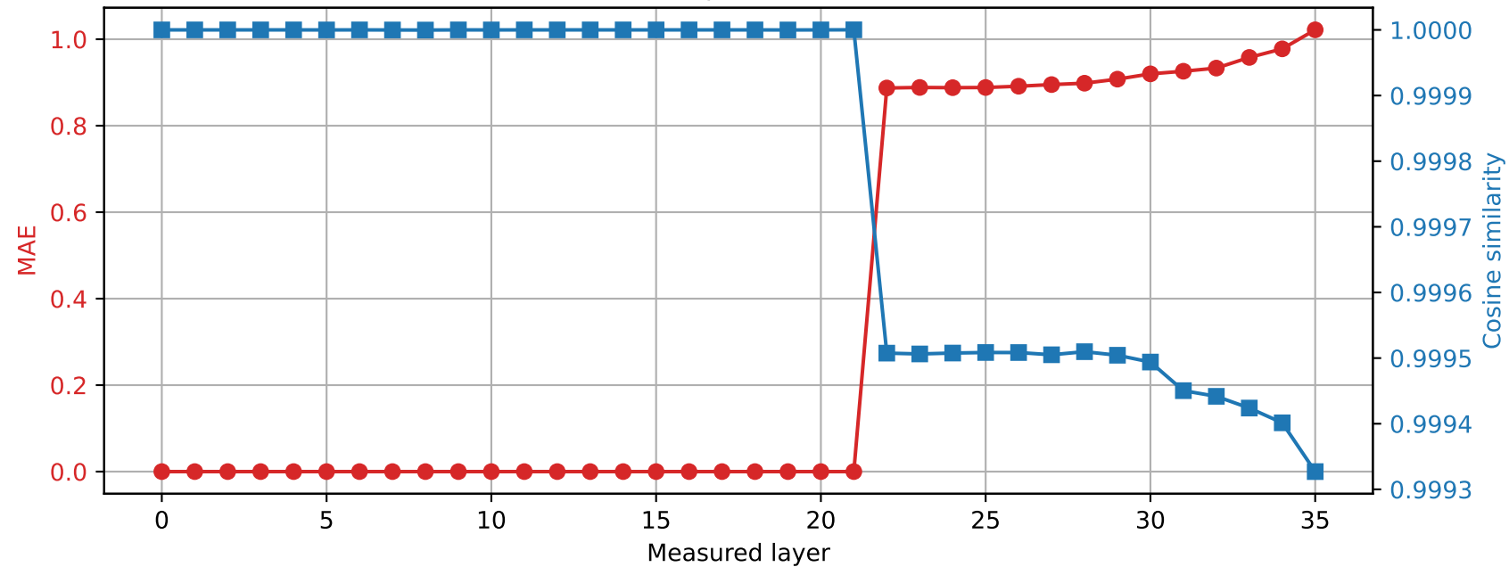
Qwen2.5-3B | Prompt 3 Spared layer 21 | Hybrid vs quantized
