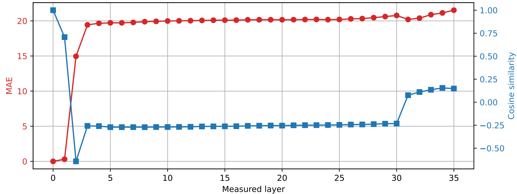
Qwen2.5-3B | Prompt 3 Spared layer 23 | Hybrid vs unquantized
