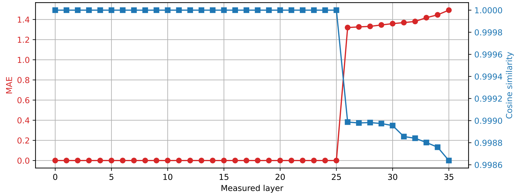
Qwen2.5-3B | Prompt 3 Spared layer 25 | Hybrid vs quantized
