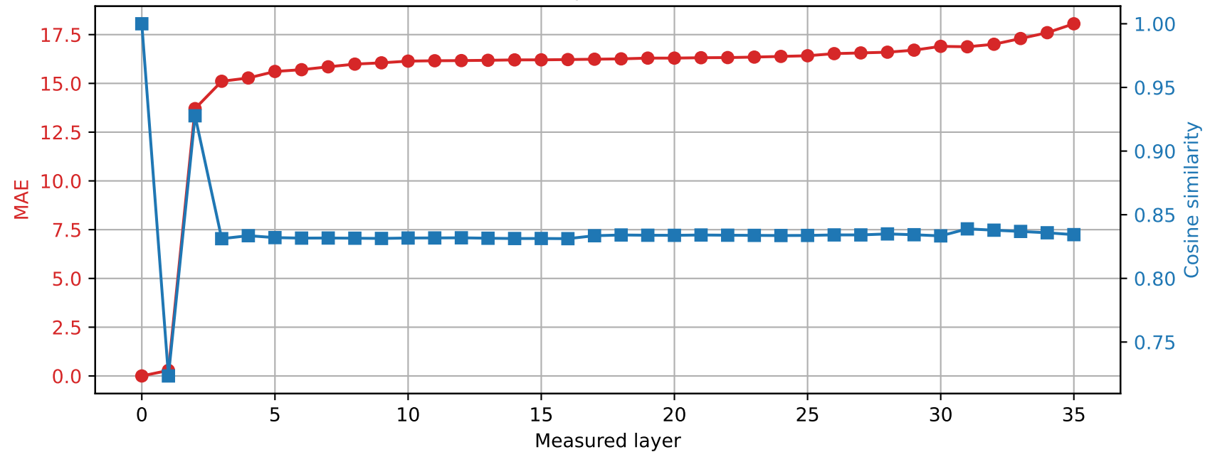
Qwen2.5-3B | Prompt 4 Spared layer 0 | Hybrid vs quantized
