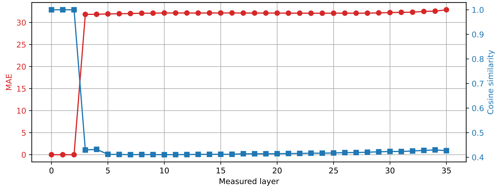
Qwen2.5-3B | Prompt 4 Spared layer 2 | Hybrid vs quantized
