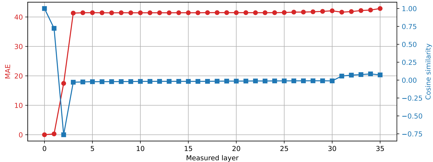
Qwen2.5-3B | Prompt 4 Spared layer 2 | Hybrid vs unquantized
