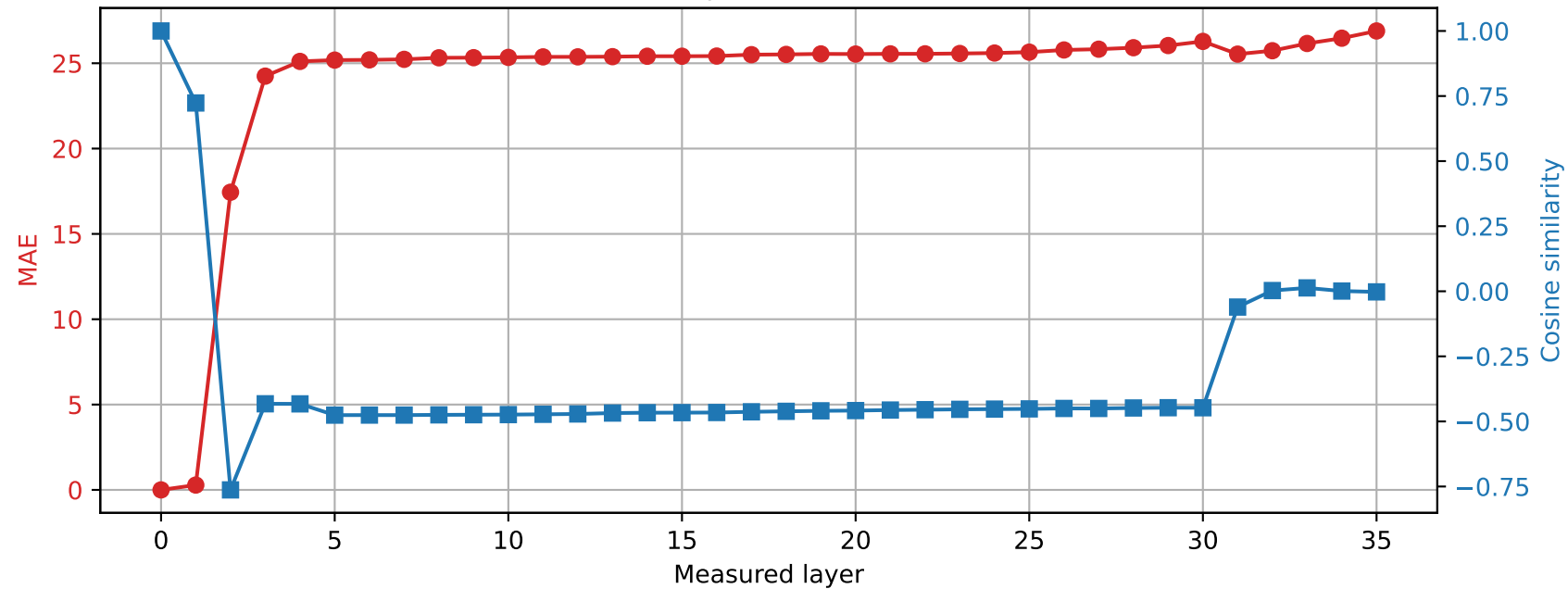
Qwen2.5-3B | Prompt 4 Spared layer 3 | Hybrid vs unquantized
