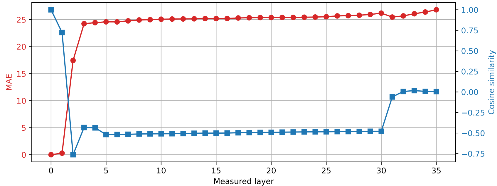
Qwen2.5-3B | Prompt 4 Spared layer 5 | Hybrid vs unquantized
