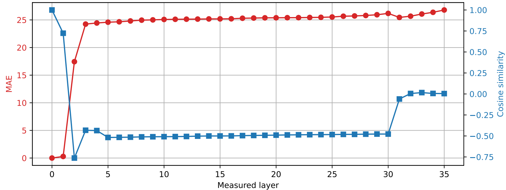
Qwen2.5-3B | Prompt 4 Spared layer 19 | Hybrid vs unquantized
