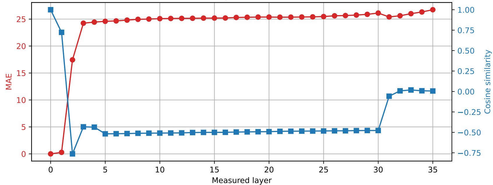
Qwen2.5-3B | Prompt 4 Spared layer 20 | Hybrid vs unquantized
