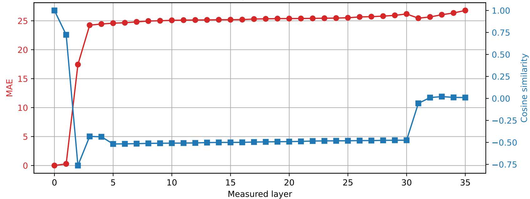
Qwen2.5-3B | Prompt 4 Spared layer 21 | Hybrid vs unquantized
