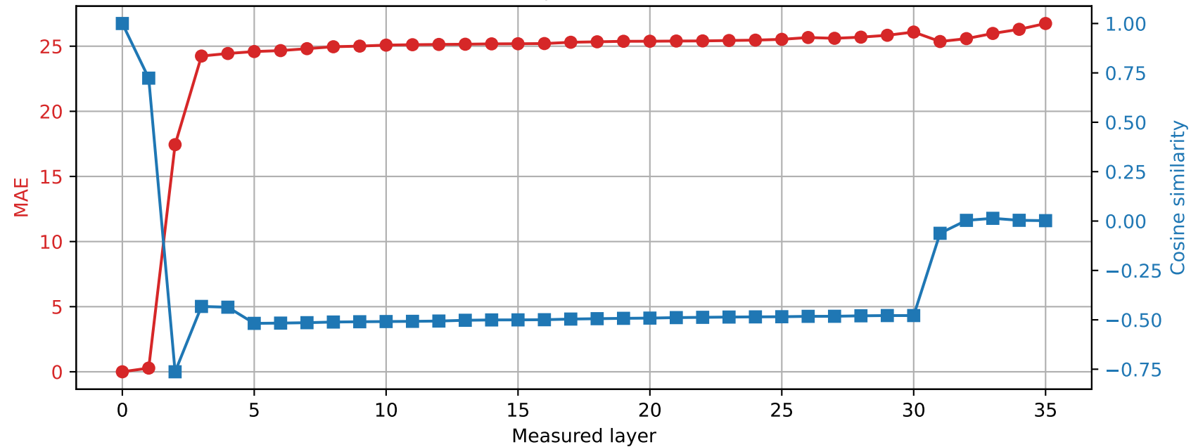
Qwen2.5-3B | Prompt 4 Spared layer 26 | Hybrid vs unquantized
