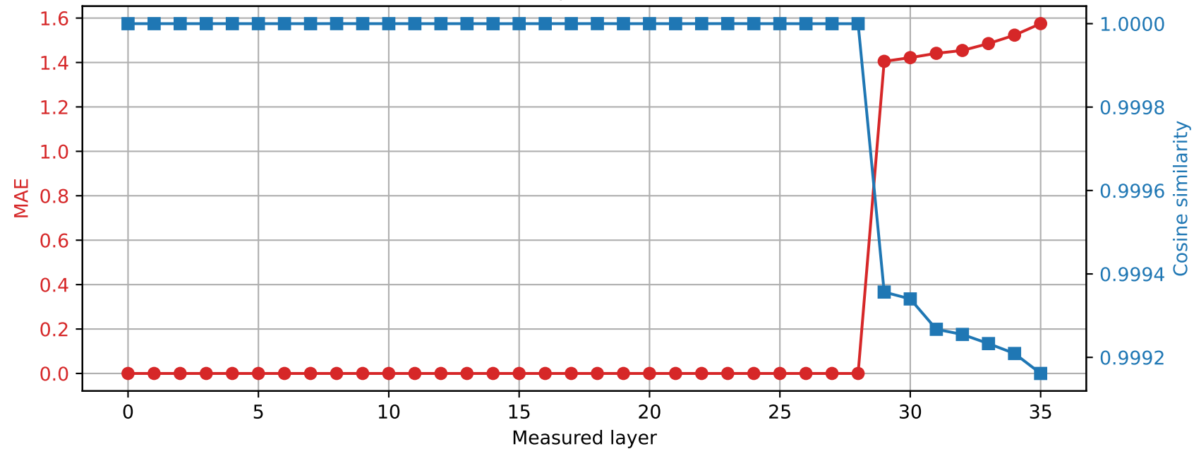
Qwen2.5-3B | Prompt 4 Spared layer 28 | Hybrid vs quantized
