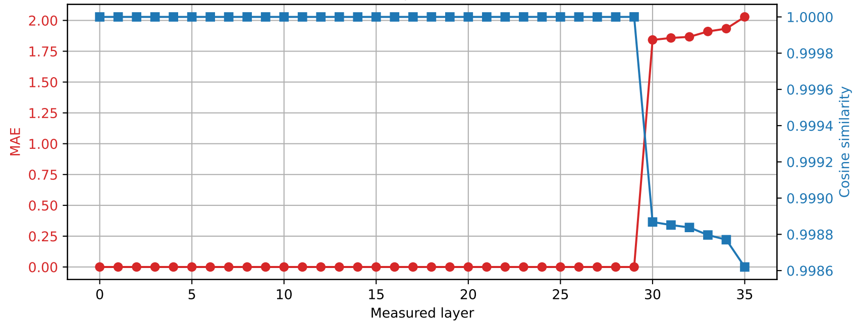
Qwen2.5-3B | Prompt 4 Spared layer 29 | Hybrid vs quantized
