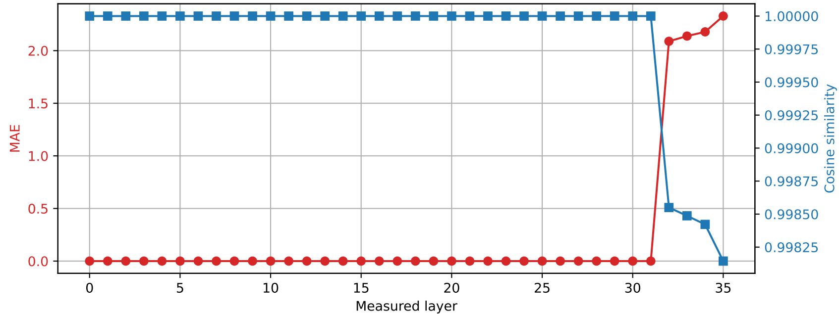
Qwen2.5-3B | Prompt 4 Spared layer 31 | Hybrid vs quantized
