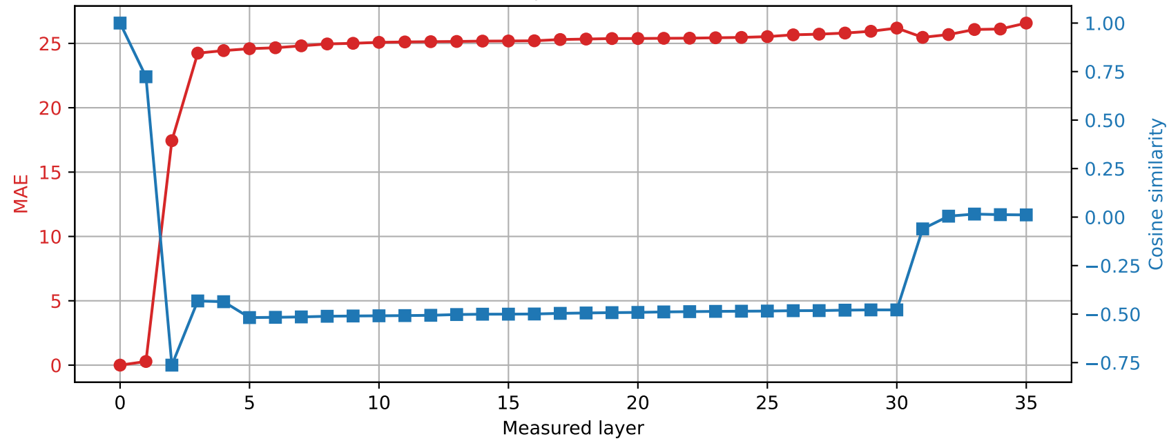
Qwen2.5-3B | Prompt 4 Spared layer 33 | Hybrid vs unquantized
