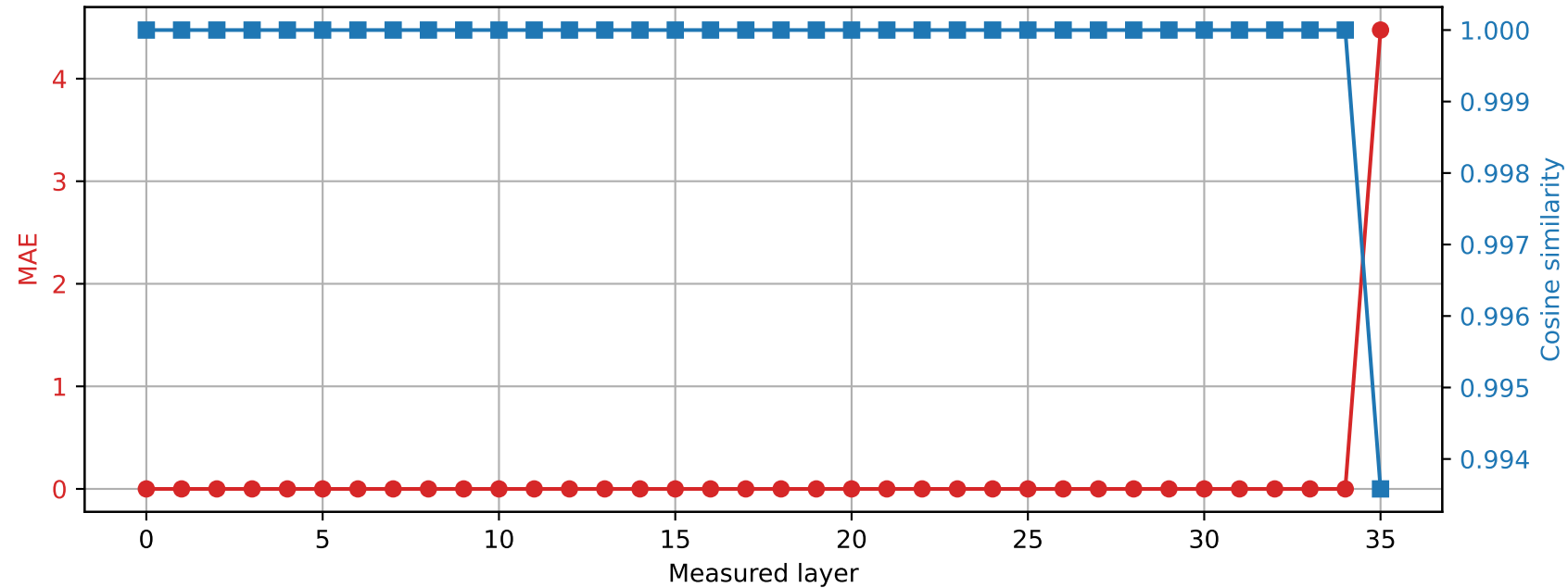
Qwen2.5-3B | Prompt 4 Spared layer 34 | Hybrid vs quantized
