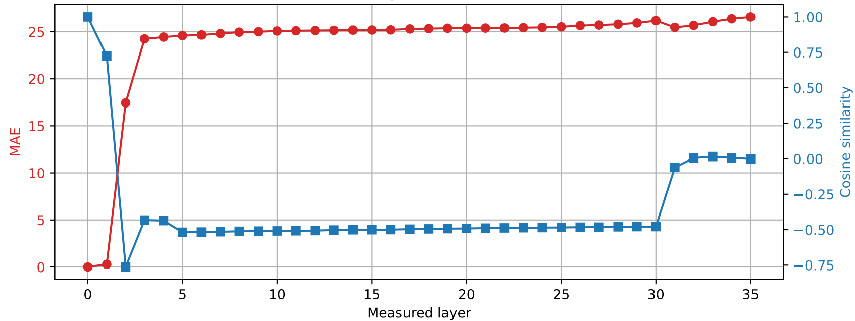
Qwen2.5-3B | Prompt 4 Spared layer 34 | Hybrid vs unquantized
