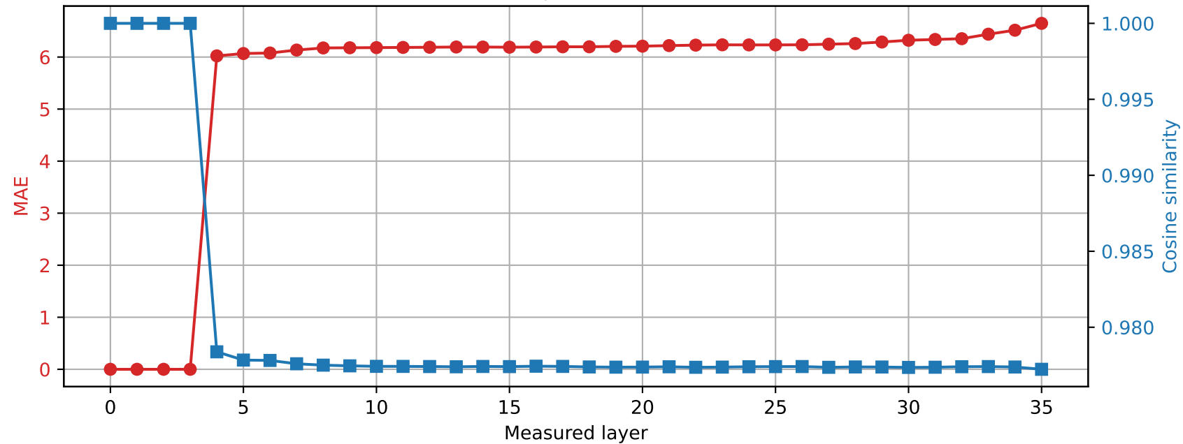
Qwen2.5-3B | Prompt 0 Spared layer 3 | Hybrid vs quantized
