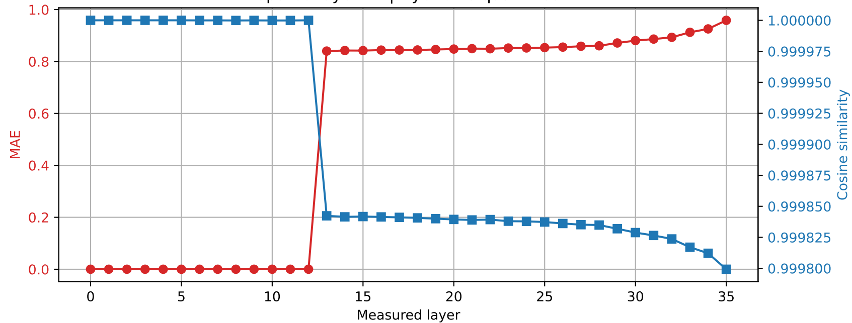
Qwen2.5-3B | Prompt 0 Spared layer 12 | Hybrid vs quantized
