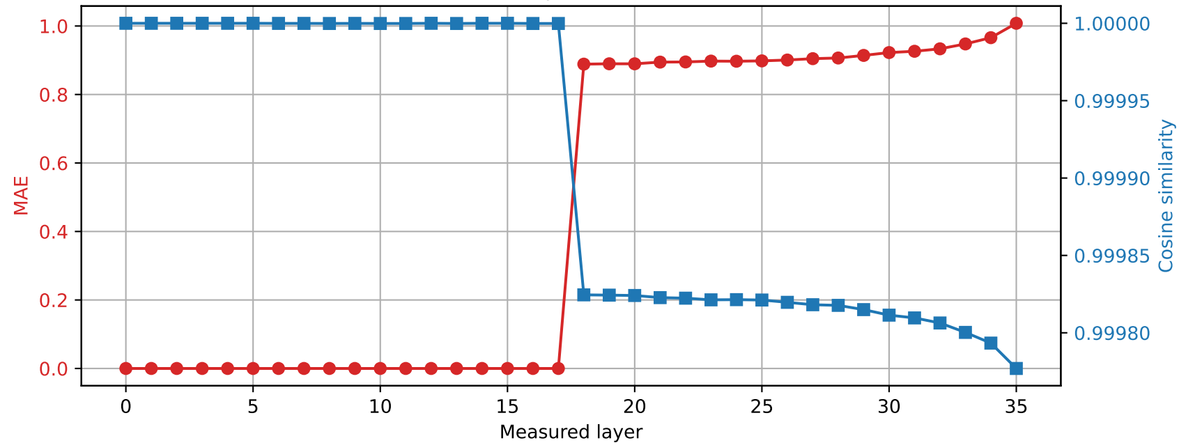
Qwen2.5-3B | Prompt 0 Spared layer 17 | Hybrid vs quantized
