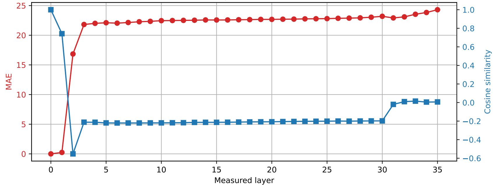
Qwen2.5-3B | Prompt 1 Spared layer 5 | Hybrid vs unquantized
