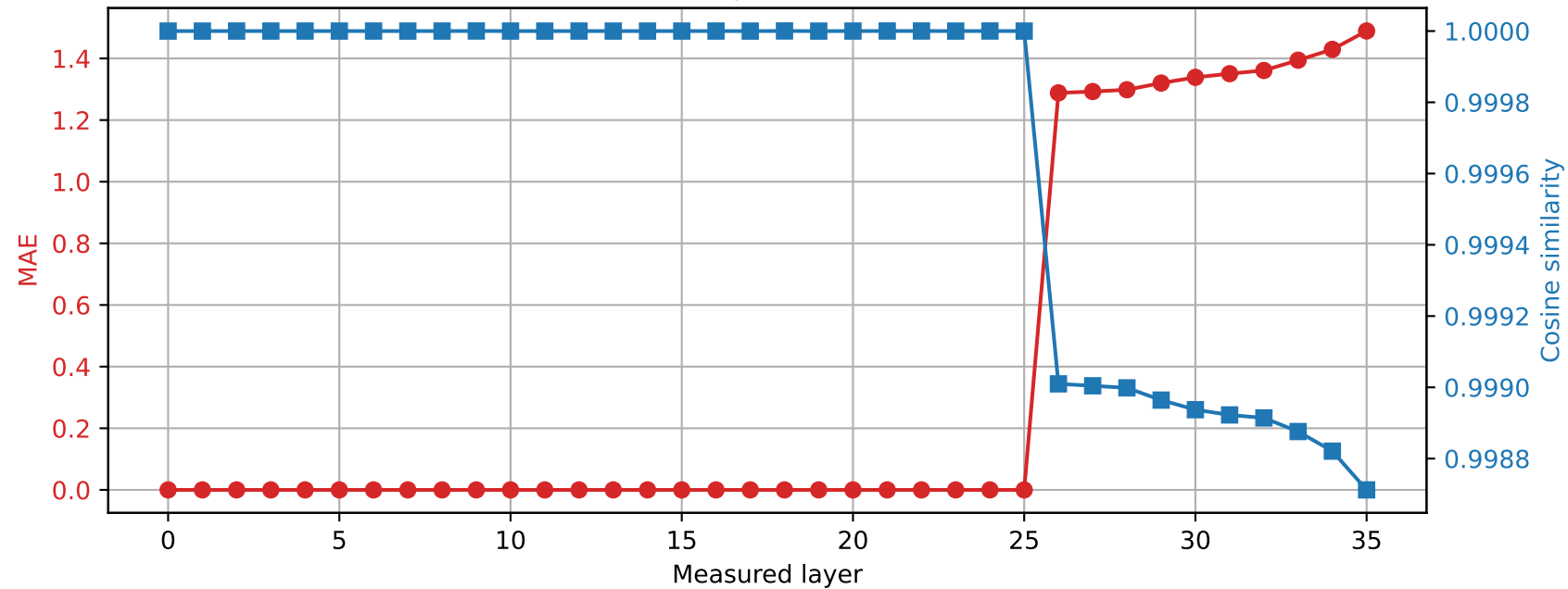
Qwen2.5-3B | Prompt 1 Spared layer 25 | Hybrid vs quantized
