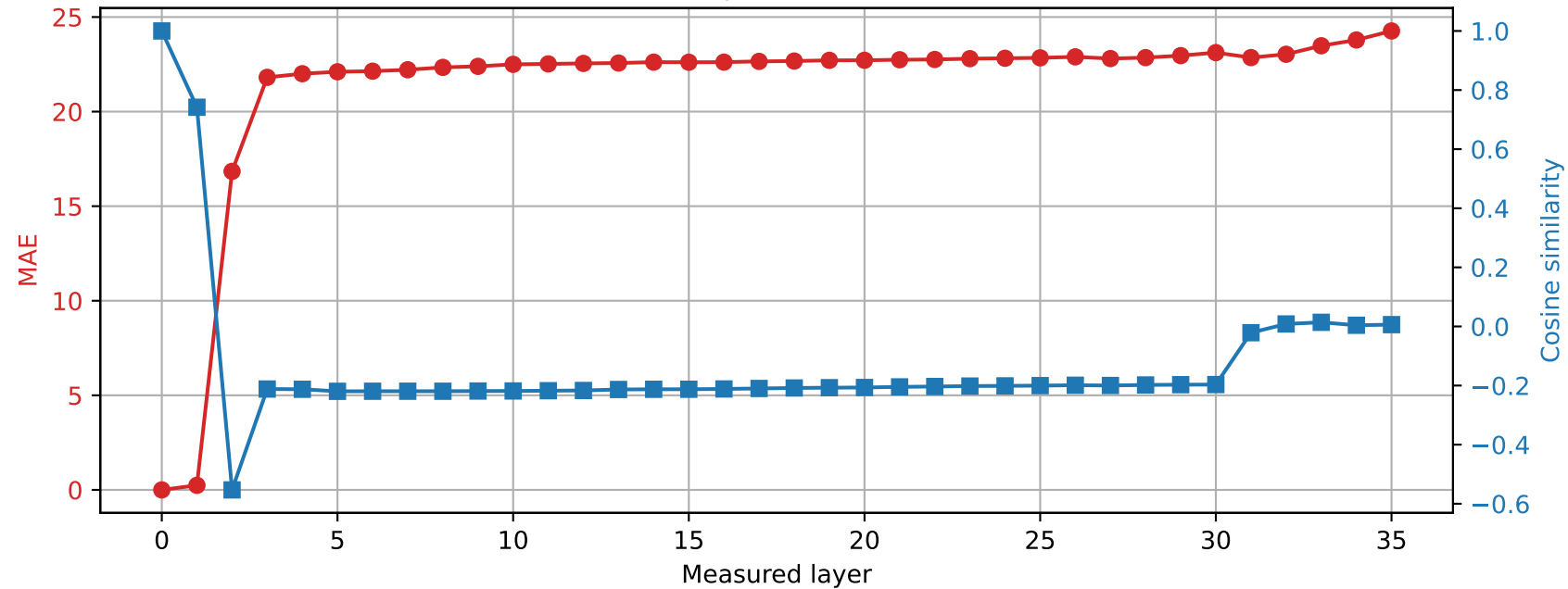
Qwen2.5-3B | Prompt 1 Spared layer 26 | Hybrid vs unquantized
