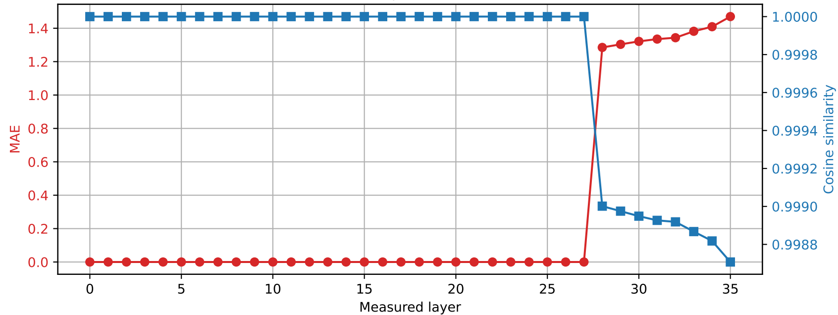
Qwen2.5-3B | Prompt 1 Spared layer 27 | Hybrid vs quantized
