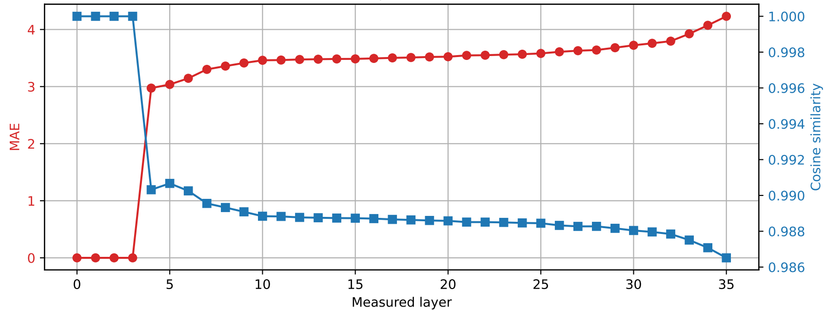
Qwen2.5-3B | Prompt 2 Spared layer 3 | Hybrid vs quantized
