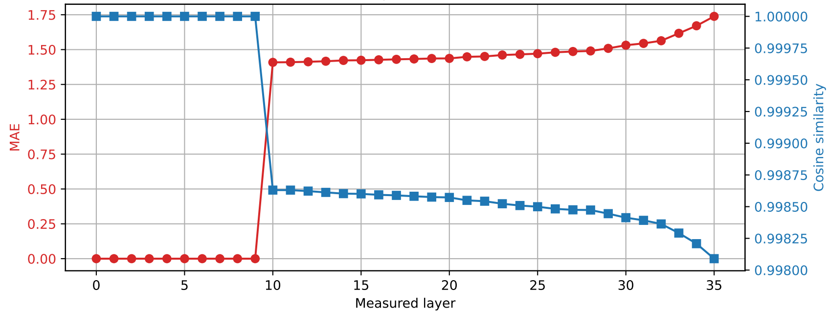
Qwen2.5-3B | Prompt 2 Spared layer 9 | Hybrid vs quantized
