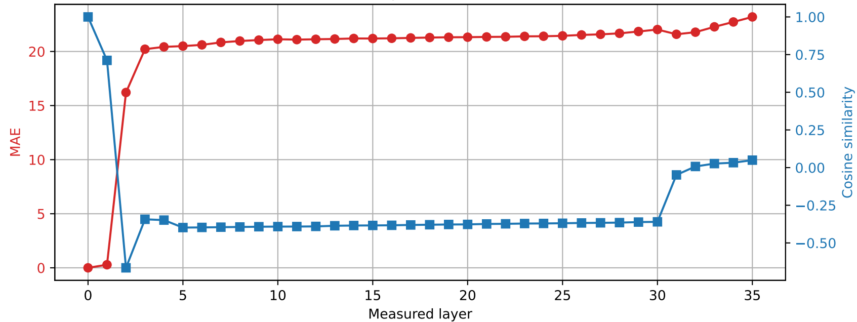
Qwen2.5-3B | Prompt 2 Spared layer 10 | Hybrid vs unquantized
